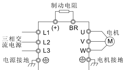
图 10-3 1K50G~22K0G/30K0P机型接制动电阻
